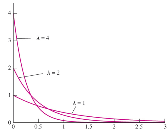
Probability Density Function
