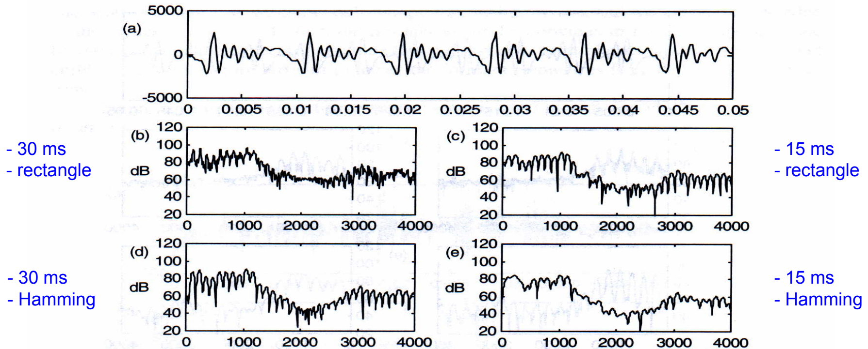
Figure 6.3 Short-time spectrum of male voiced speech (vowel /ah/ with local pitch of 110Hz): (a) time signal, spectra obtained with (b) 30 ms rectangular window and (c) 15 ms rectangular window, (d) 30 ms Hamming window, (e) 15 ms Hamming window. The window lobes are not visible in (e), since the window is shorter than 2 times the pitch period. Note the spectral leakage present in (b).
