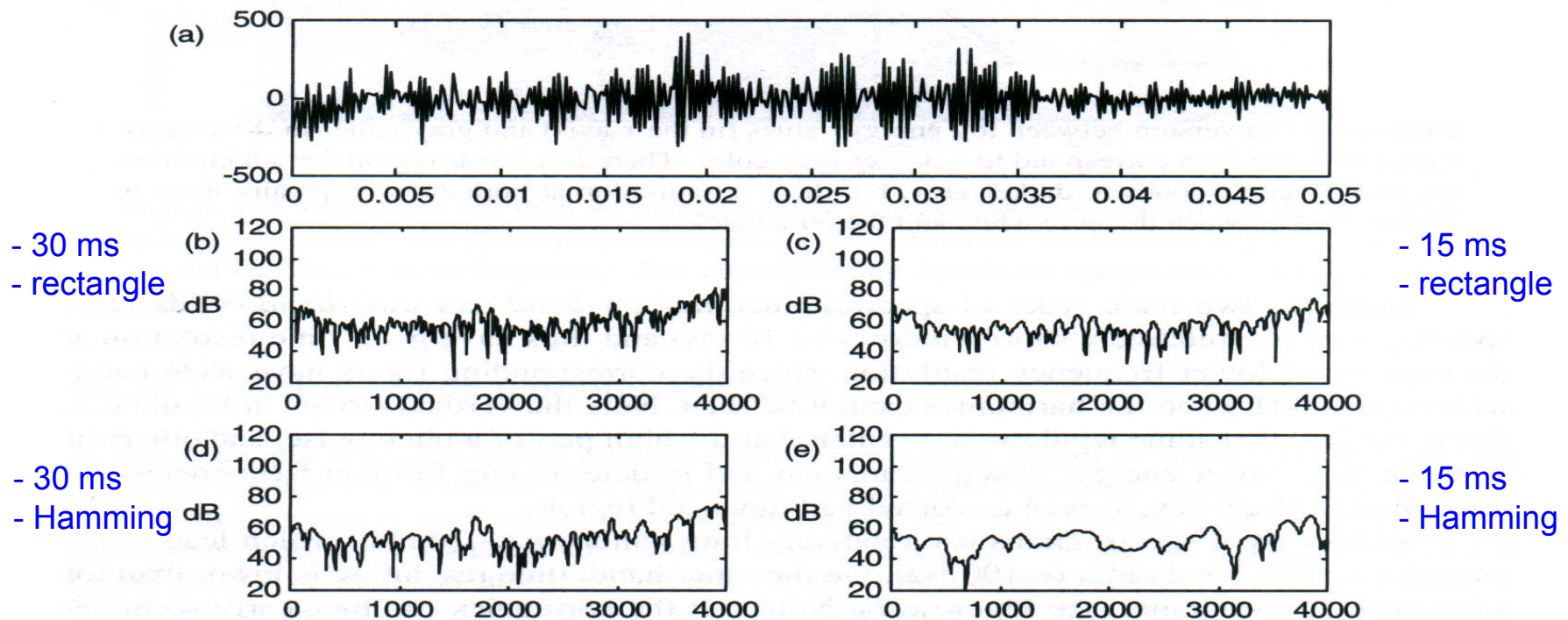
Figure 6.5 Short-time spectrum of unvoiced speech: (a) time signal, (b) 30 ms rectangular window, (c) 15 ms rectangular window, (d) 30 ms Hamming window, (e) 15 ms Hamming window.
